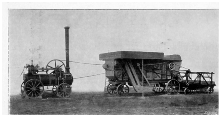
RUSTON AND PROCTOR'S THRASHING PLANT
